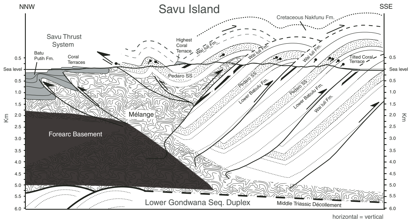
Figure 9. Composite north-northwest-south-southeast section across Savu (see Fig. 3 for line of section). The structure of northern section is according to seismic profiles off the north coast and from drilling data. Folds and thrust faults are determined from field mapping (Fig. 3). Dip measurements are given by black dots with line pointing in direction of dip. Black bodies in Wai Luli Formation are basalt. Detachment depth is estimated from the projected depth of the Sumba Ridge and stratigraphic thickness of units incorporated into thrust sheets. Cretaceous units are interpreted as a roof thrust for the Upper Triassic–Jurassic duplex. Assuming no subduction erosion, the southern edge of the forearc was the precollisional Sunda-Banda trench, which is now abandoned due to accretion of Australian continental margin in front and beneath it. SS—sandstone; Seq.—sequence.
